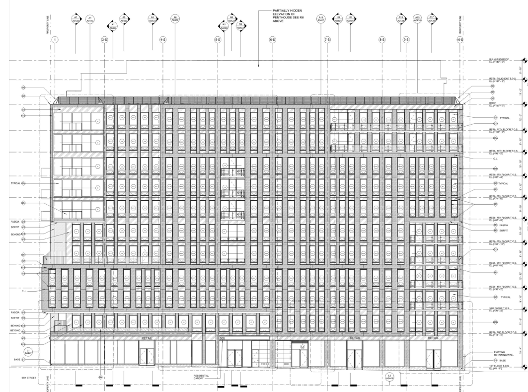
2. South Elevation
